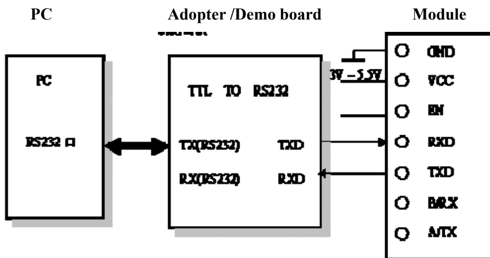
RF-Magic Setup Connecting Drawing
